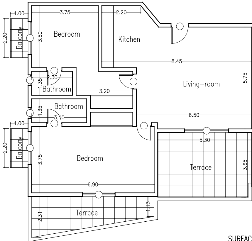
Apartment T3-3 (level 1)
